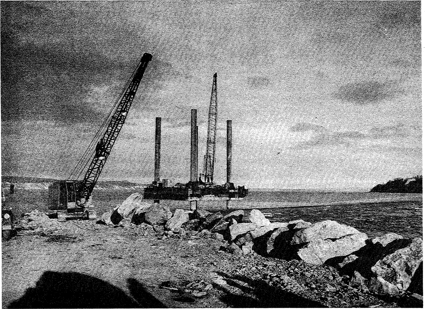
LARGE PILINGS STAND READY TO BE DRIVEN DEEP INTO THE HEART OF THE COOK INLET'S MUDDY BOTTOM AS THE FIRST SECTION OF THE NEW DOCK TAKES SHAPE.
