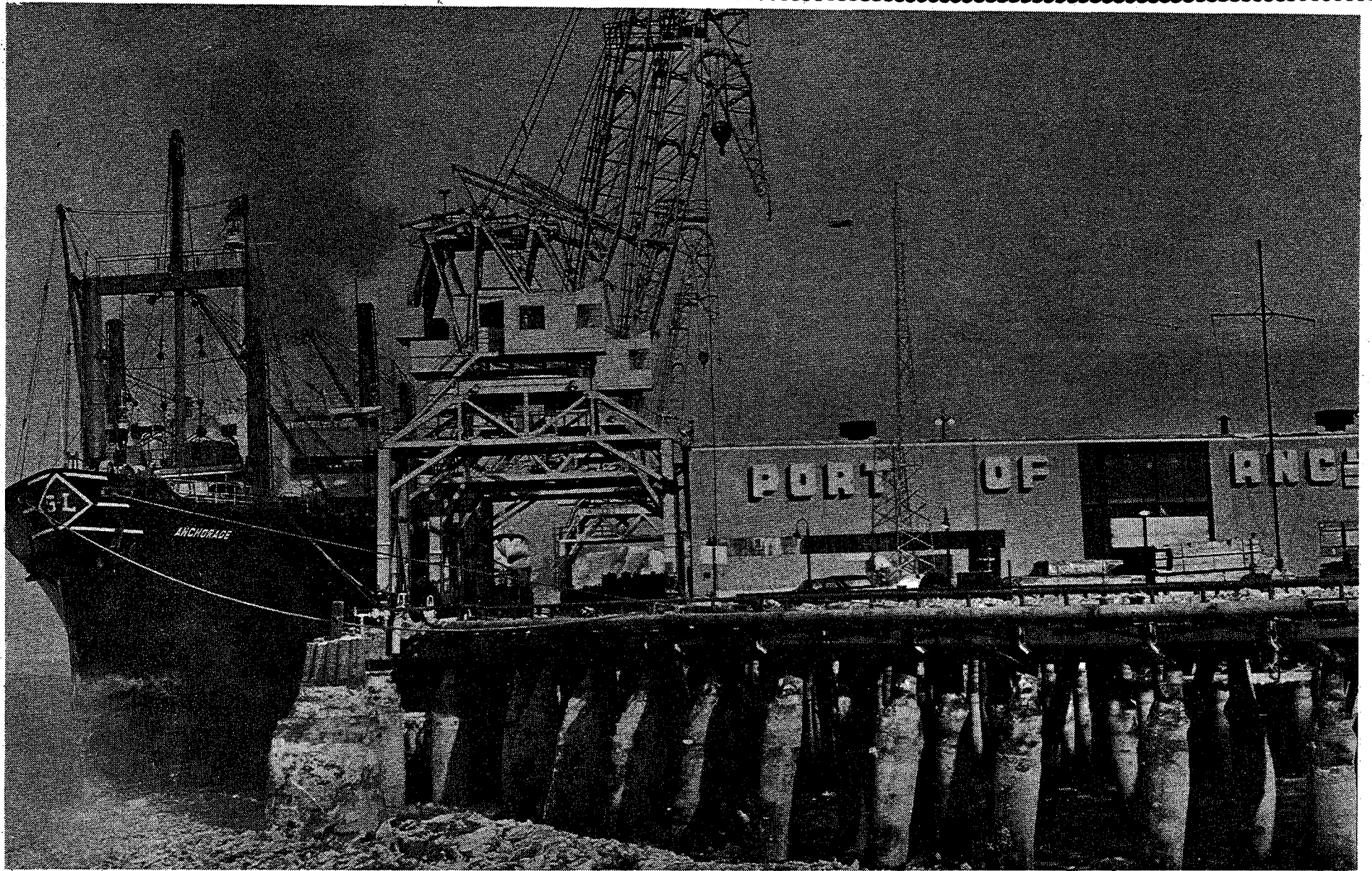
WINTER ICE DOESN'T SLOW THE PACE MUCH AT ALASKA'S BUSIEST AND MOST MODERN PORT. ICE FORMS AROUND SPECIALLY DESIGNED PILING TO FORM LARGE FROZEN BOTTLES.
